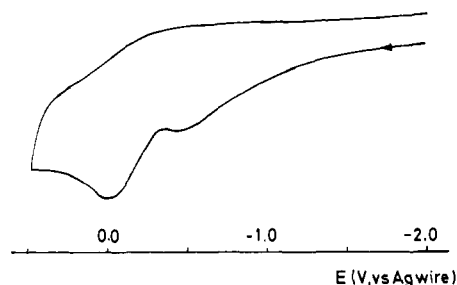
Figure 5. Cyclic voltammogram of the solution obtained by reduction of allyl iodide ( 1a ) or bromide ( 1b ) with solvated electrons in 0.3 M KI in liquid ammonia at platinum at -75 °C.
